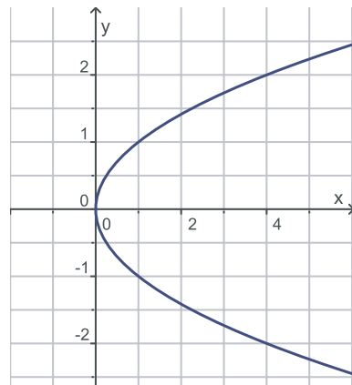
y^2 = x
